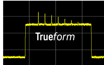
While DDS technology may skip points at higher frequencies, Trueform never skips points and is always anti-aliased.
