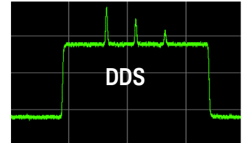
While DDS technology may skip points at higher frequencies, Trueform never skips points and is always anti-aliased.
